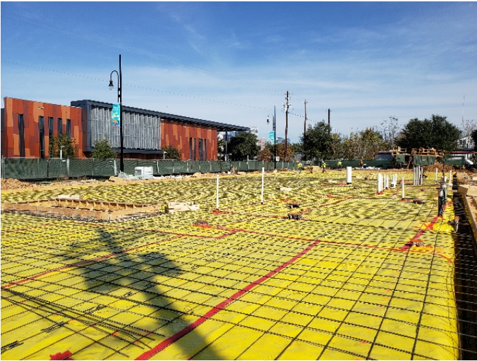
Prepped building slab for concrete (12/10/19)
