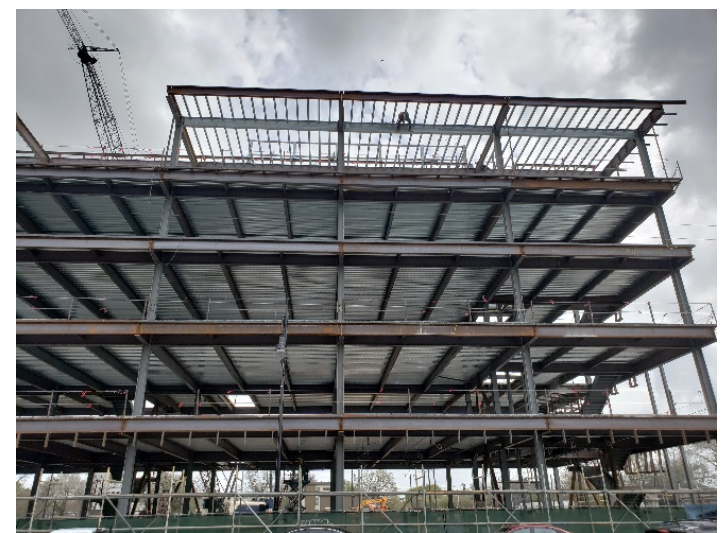
Roof steel framing being installed for office building (03/16/20)
